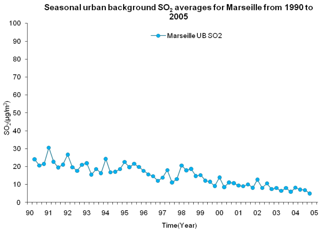
Figure 15 – Plot of seasonal urban background SO 2 averages for Marseille from 1990 – 2001
